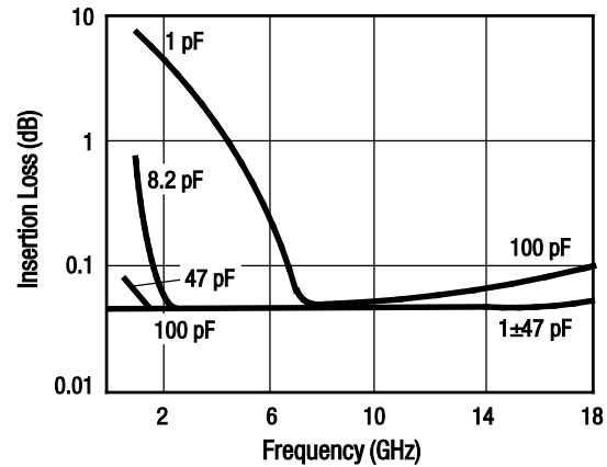
Figure 1. Typical Insertion Loss vs Frequency (50 \Omega System)
