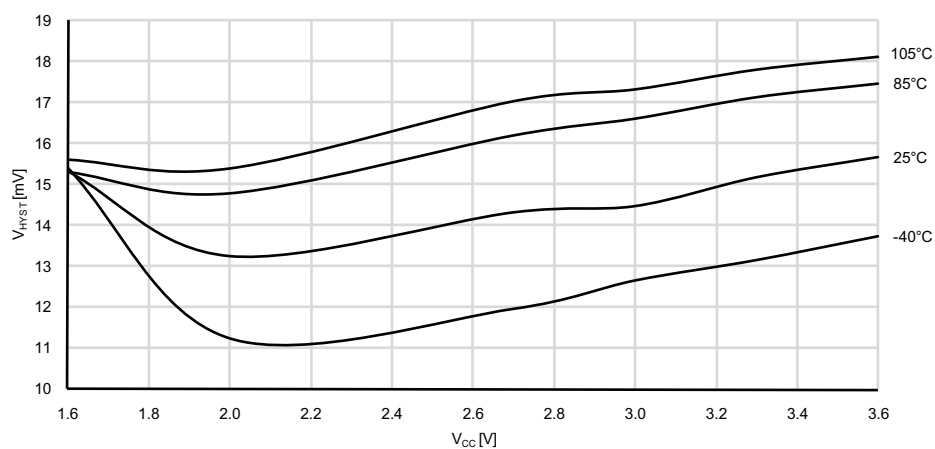
Figure 36-41. Analog Comparator Hysteresis vs. V_{CC}
