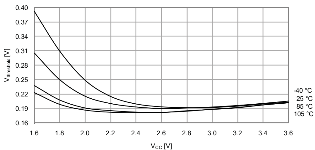
Figure 36-29. I/O Pin Input Hysteresis vs. V_{CC}
