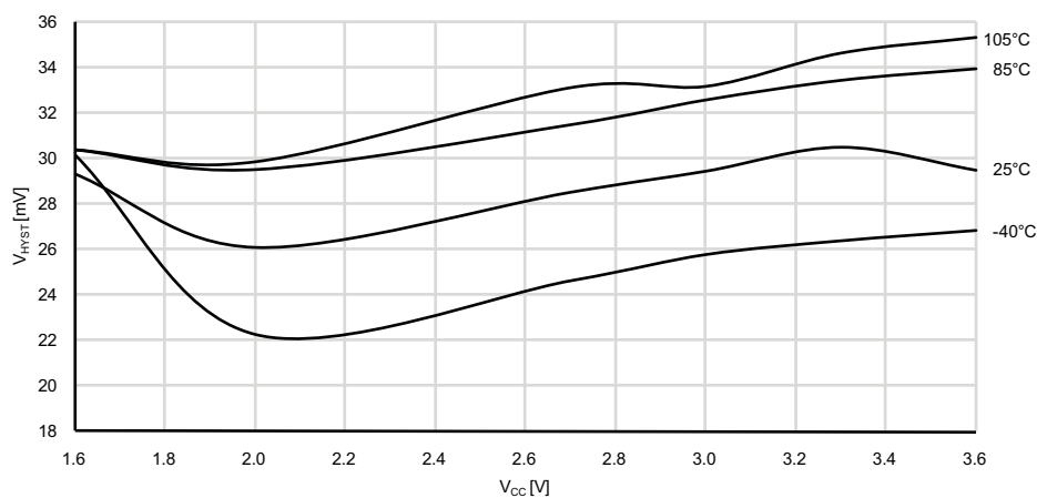
Figure 36-42. Analog Comparator Hysteresis vs. V_{CC}
