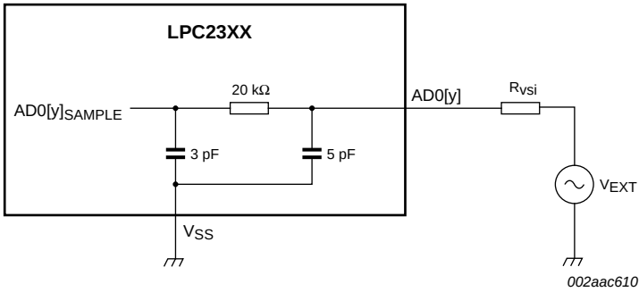
Fig 16. Suggested ADC interface - LPC2387 AD0[y] pin
