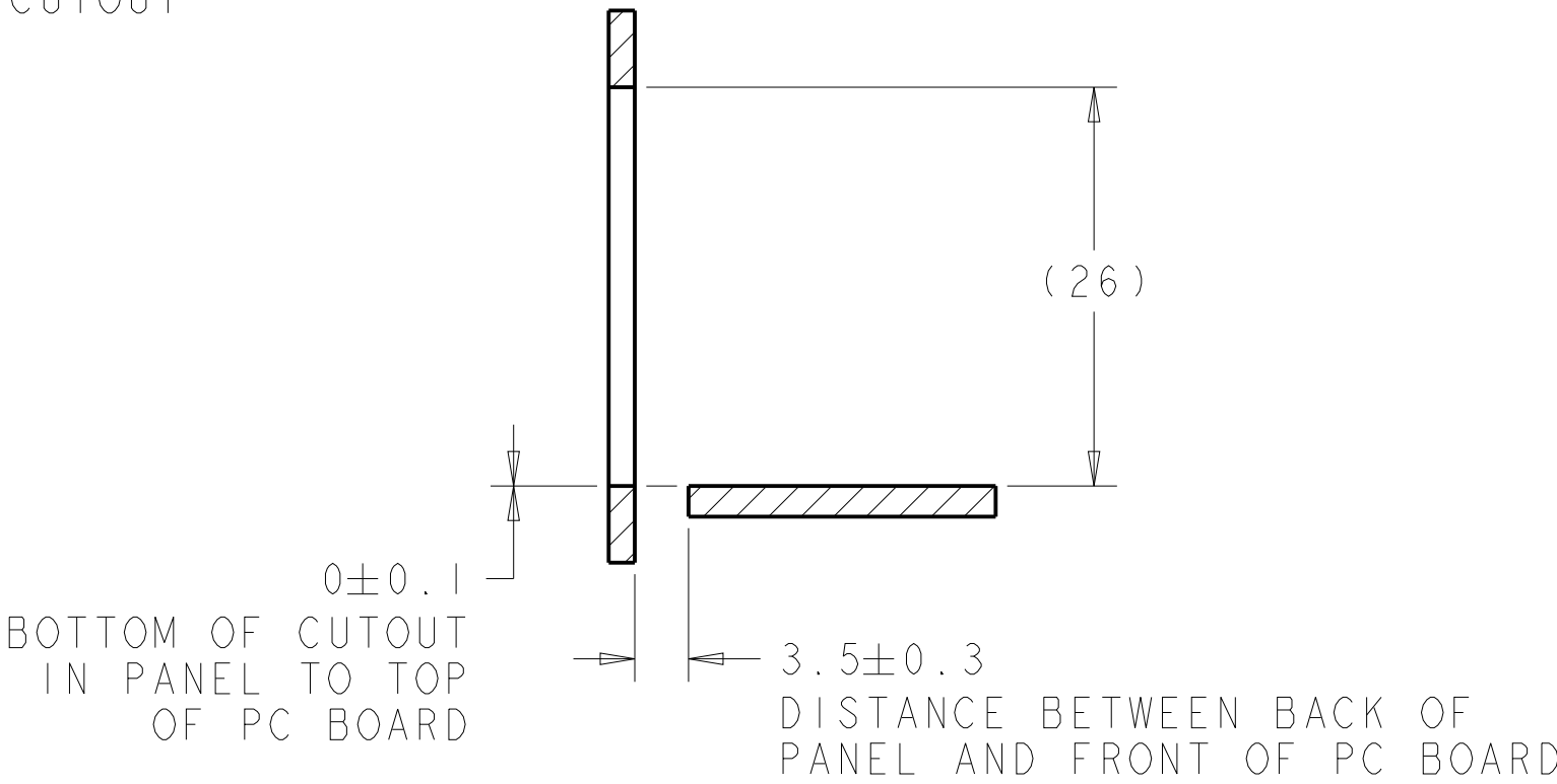
SECTION U-U
