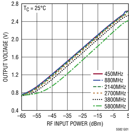
Output Voltage vs RF Input Power
