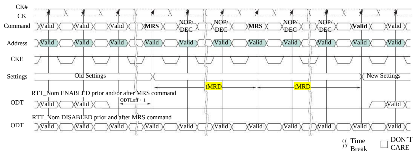
Figure 2.3.1a tMRD Timing
