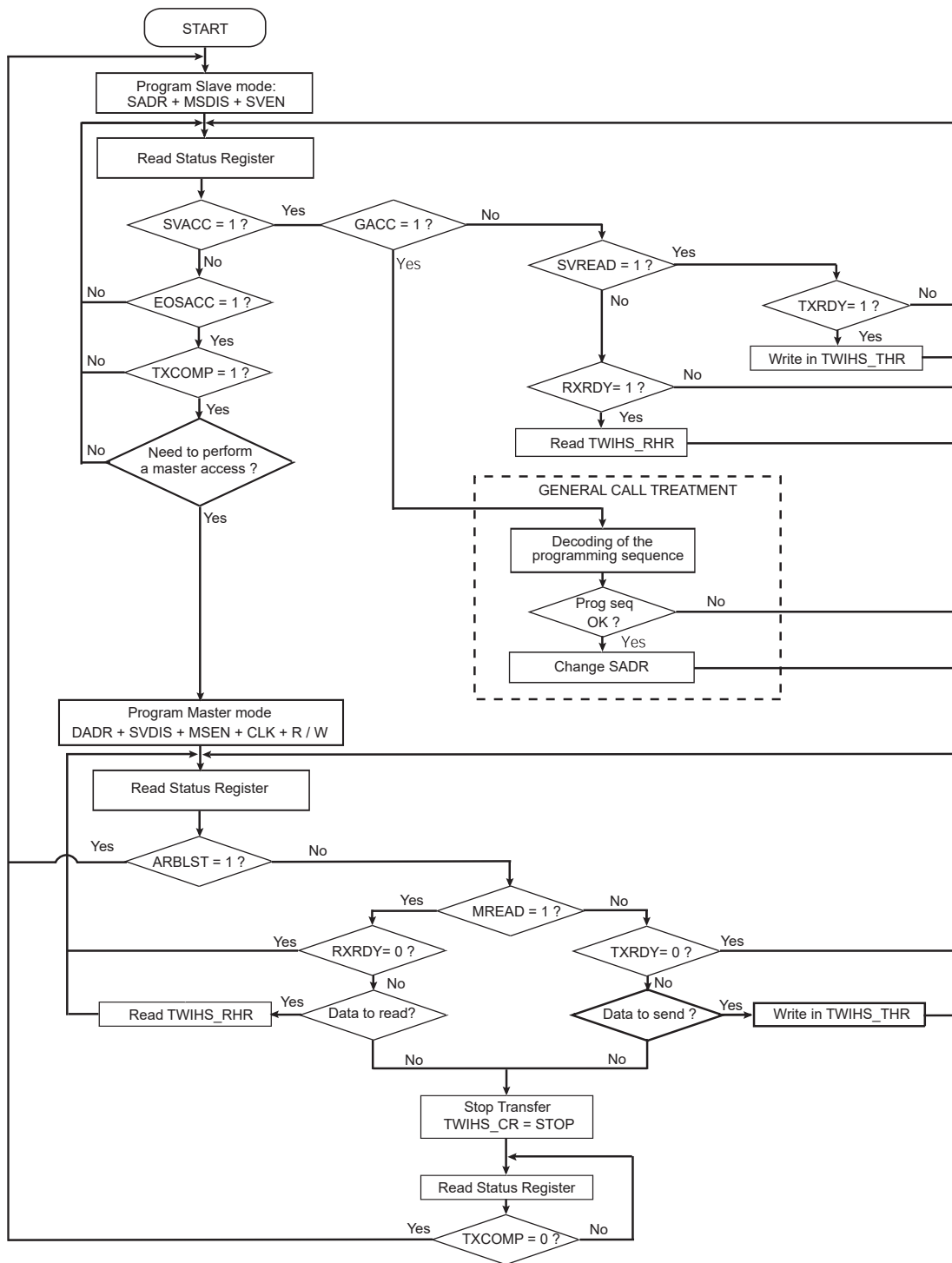
Figure 45-30. Multimaster Flowchart
