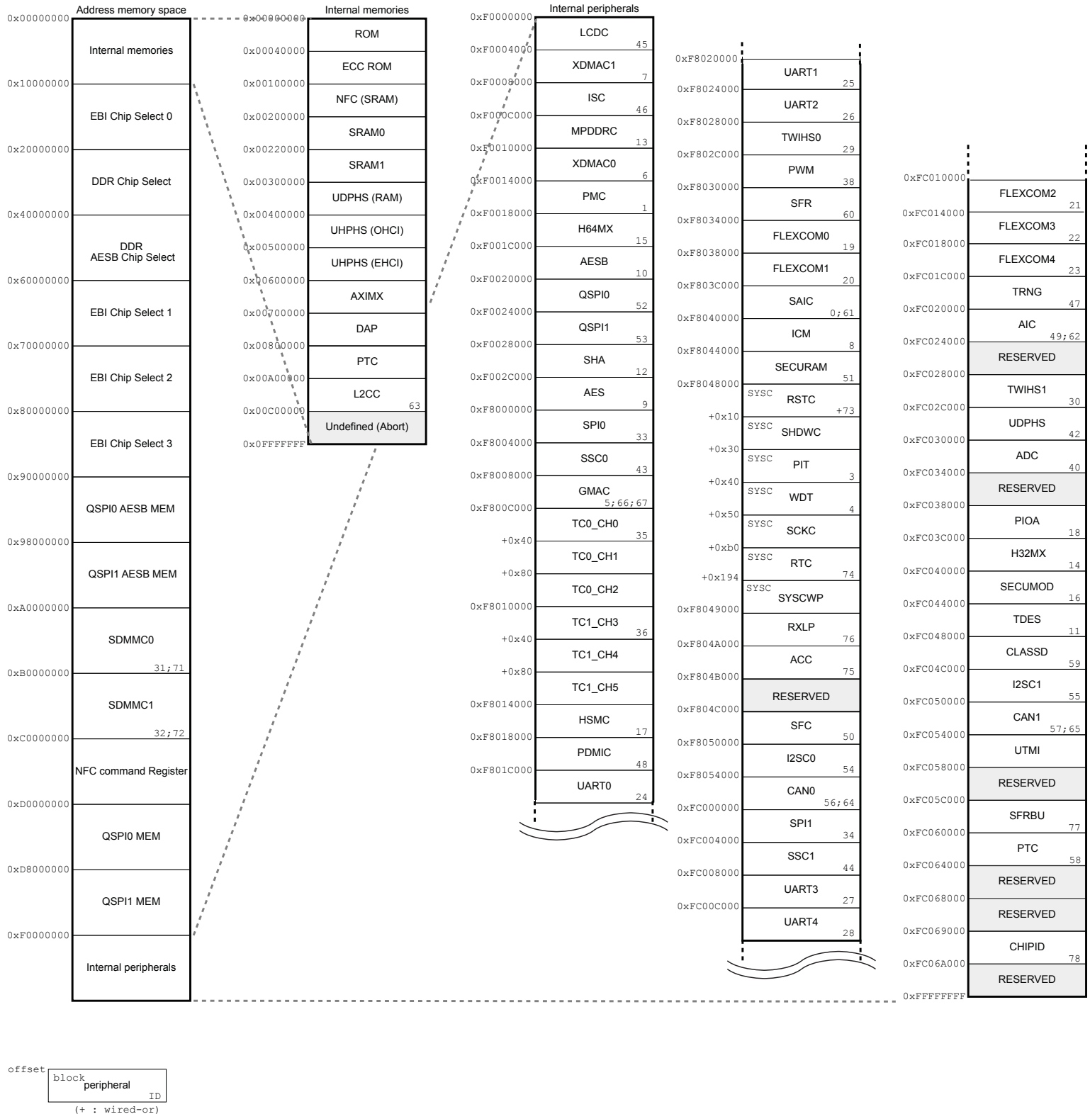
Figure 8-1. Memory Mapping
