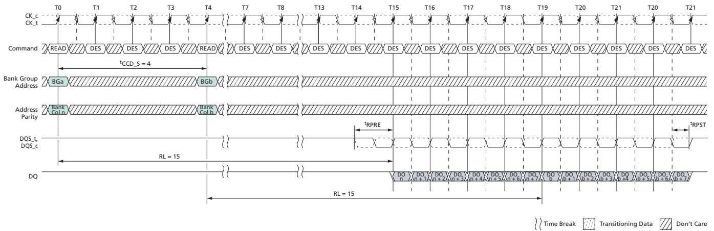
Figure 158: Consecutive READ (BL8) with 1 st CK Preamble and CA Parity in Different Bank Group
