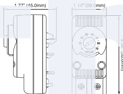
Thermostat Dimensions
