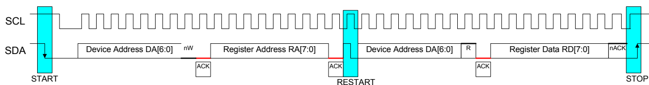
Figure 32. Read Cycle
