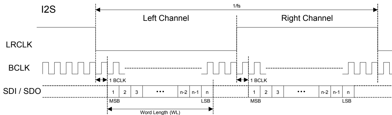
Figure 28. I 2 S Justified Audio Interface (assuming n-bit word length)
