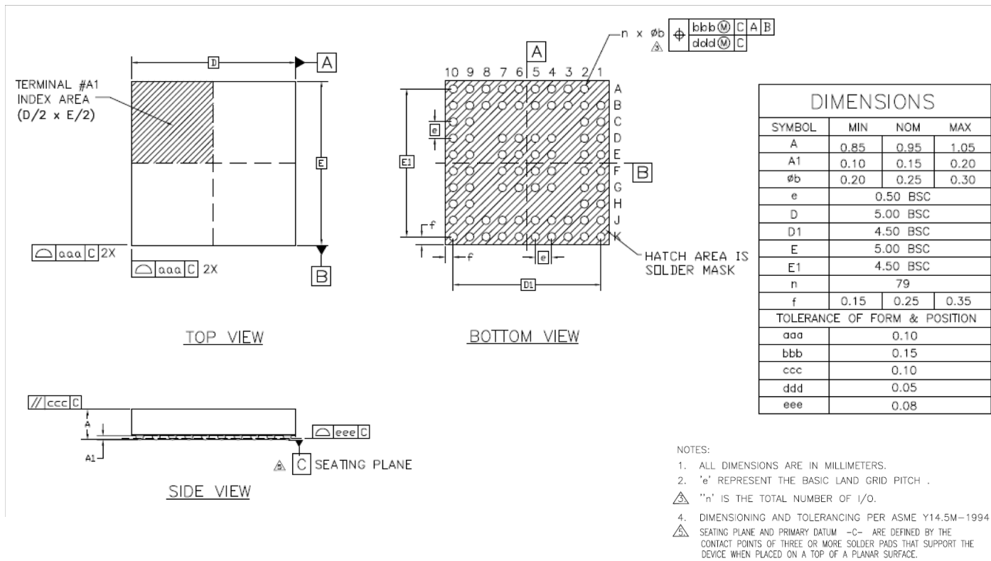
Figure 39. NAG/HLA Package Outline
