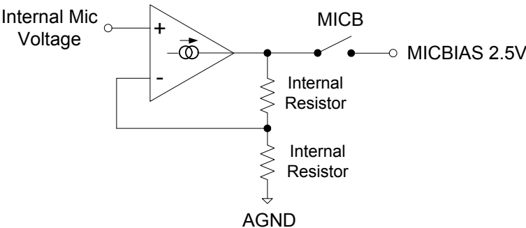
Figure 18. Mic Bias
