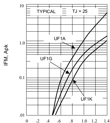
Fig. 2-FORWARD CHARACTERISTICS
