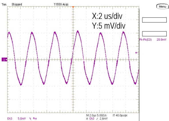
Output Ripple and Noise (Vin=12V, Vout=5.0V, Iout=6A, Cload=400uF, ScopeBW=20MHz)
