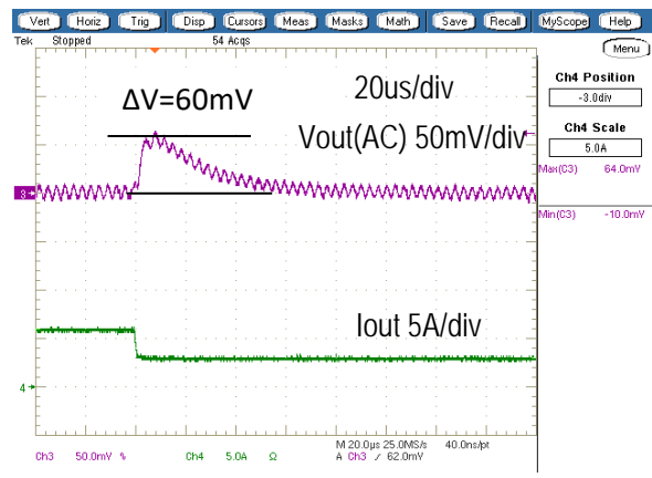
Step Load Transient Response (Vin=12V, Vout=3.3V, Cload=400uF, Iout=6A to 3A, 2.5A/us)
