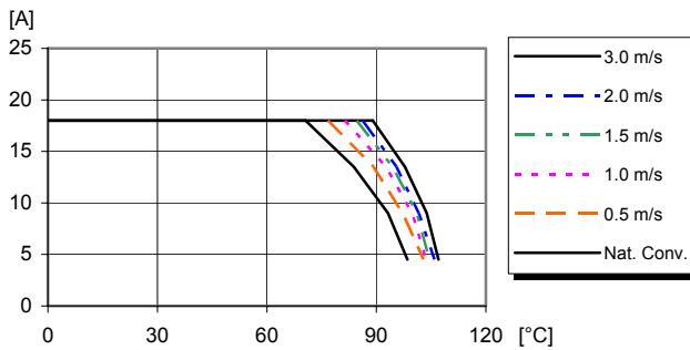
Available load current vs. ambient air temperature and airflow at V_i = 12\text{ V} . See Thermal Consideration section.
