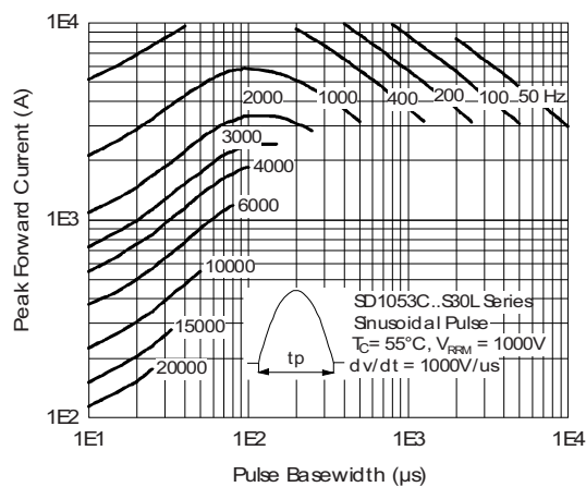
Fig. 35 - Frequency Characteristics
