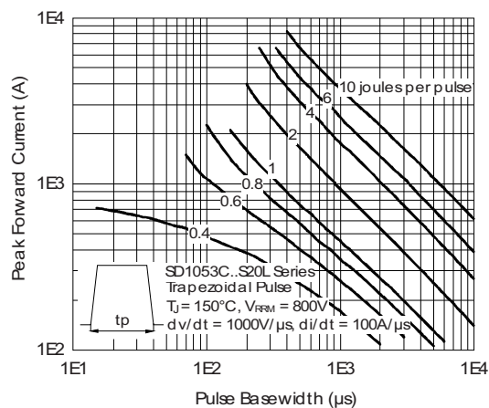
Fig. 32 - Maximum Total Energy Loss Per Pulse Characteristics
