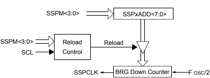
Figure 26-40. Baud Rate Generator Block Diagram
