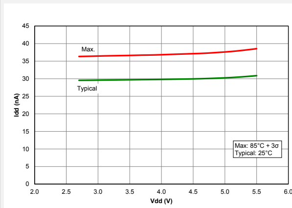
Figure 39-64. I_{PD} , Fixed Voltage Reference (FVR), PIC18F27/47K40 only
