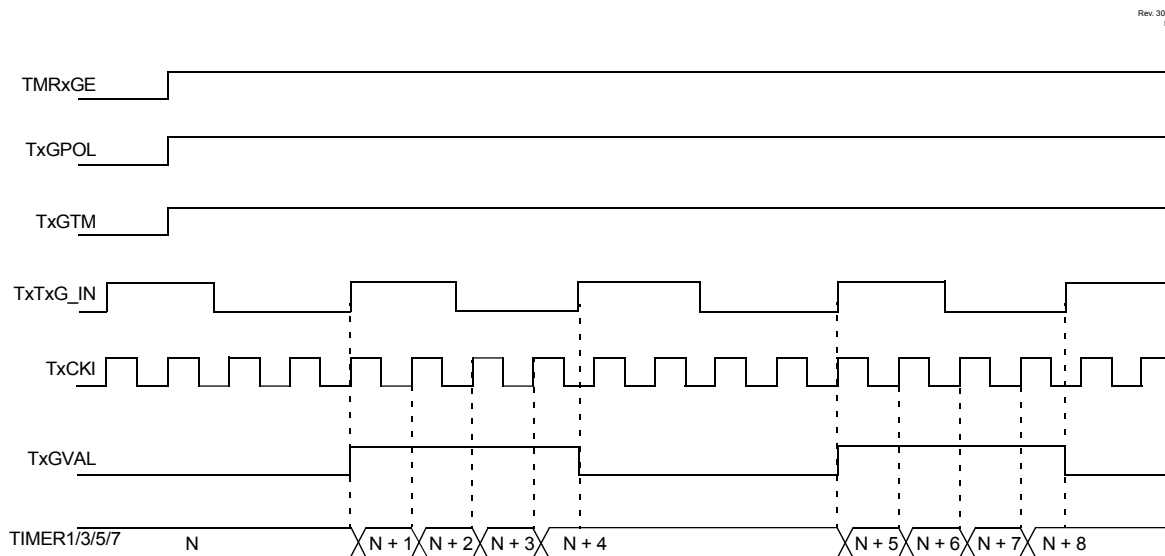
Figure 19-5. TIMER1 GATE TOGGLE MODE
