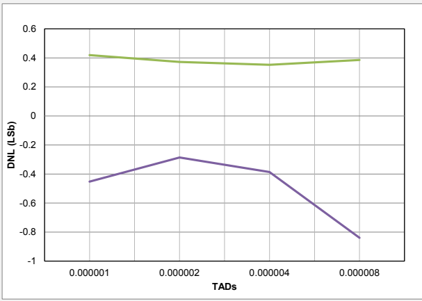
Figure 39-6. ADC, Single-Ended DNL, V_{DD} = 3.0V , V_{REF} = 3.0V
