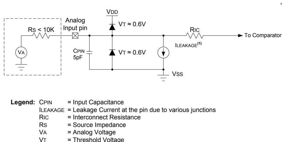
Figure 32-3. Analog Input Model
