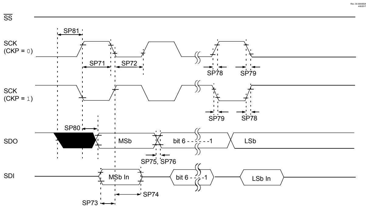
Figure 38-16. SPI Master Mode Timing (CKE = 0, SMP = 0)
