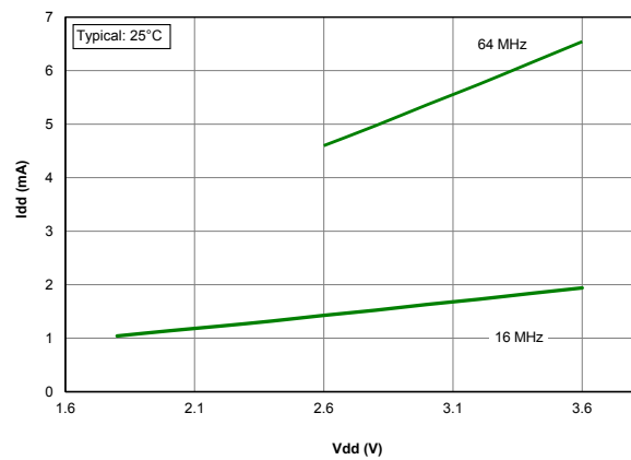
Figure 39-51. I_{DD} , ECH Oscillator, Typical, PIC18LF27/47K40 only
