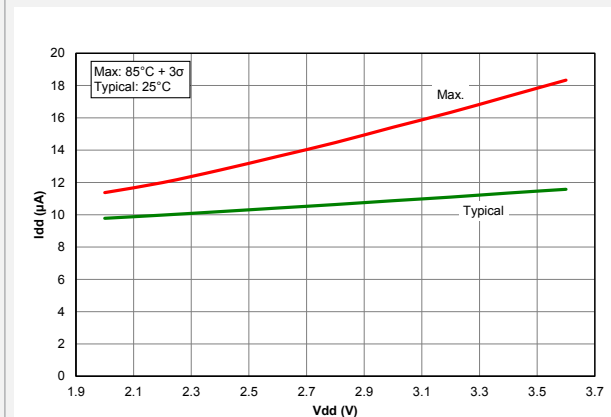
Figure 39-65. I_{PD} , Brown-out Reset, BORV = 1, PIC18LF27/47K40 only
