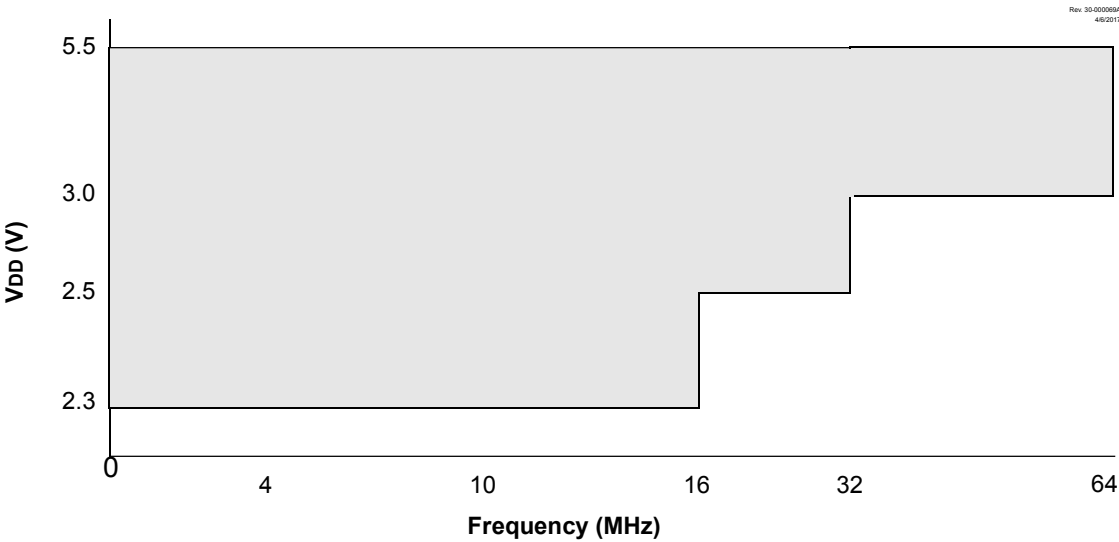
Figure 38-1. Voltage Frequency Graph, -40°C ≤ T A ≤ +125°C, for PIC18F27/47K40 only
