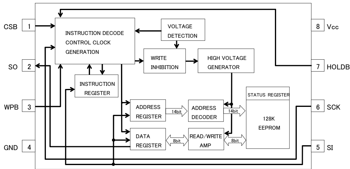
Figure 3. Block Diagram
