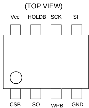
Figure 4. Pin Configuration
