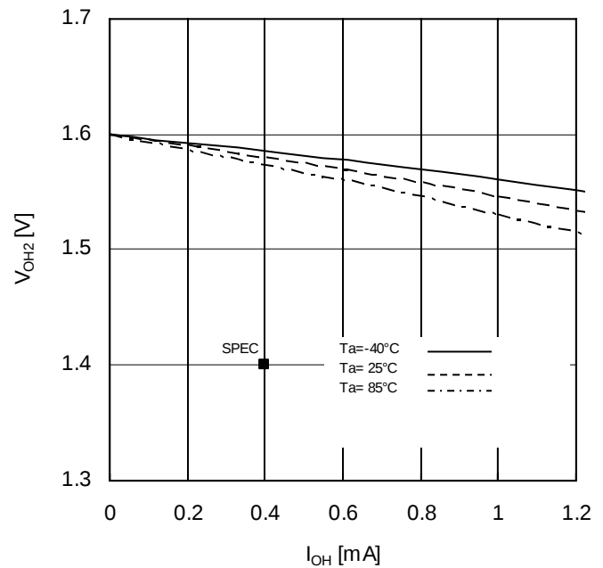
Figure 10. Output High Voltage2 vs Output Current (Vcc=1.6V)
