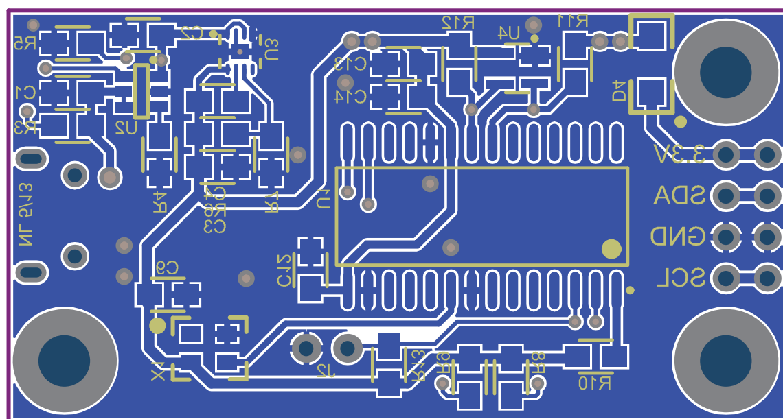
Figure 4. DS3900P2 PCB Layout—Bottom
