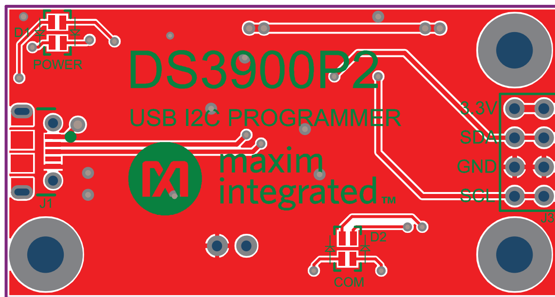
Figure 3. DS3900P2 PCB Layout—Top
