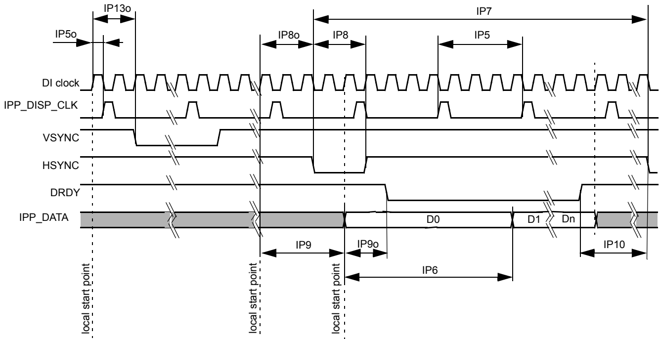
Figure 48. TFT Panels Timing Diagram—Horizontal Sync Pulse
