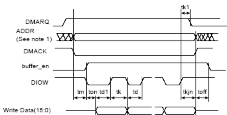
Figure 69. MDMA Write Timing Diagram
