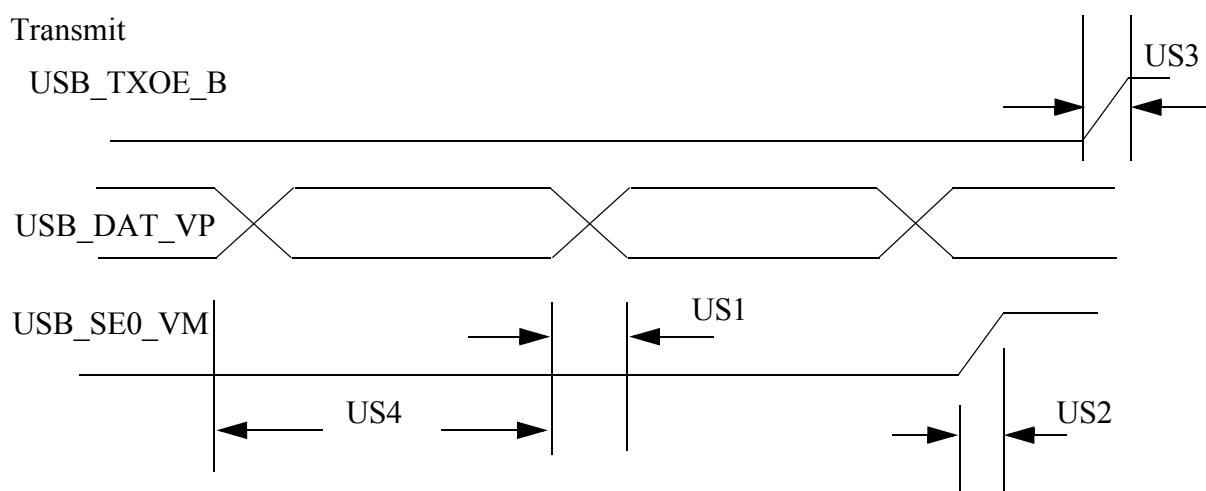
Figure 91. USB Transmit Waveform in DAT_SE0 Bidirectional Mode
