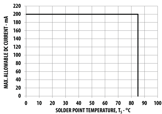
Figure 16: Maximum Forward Current vs. Solder Point Temperature. Derated based on T_{JMAX} = 110^{\circ}C , R_{\theta J-S} = 20^{\circ}C/W .
