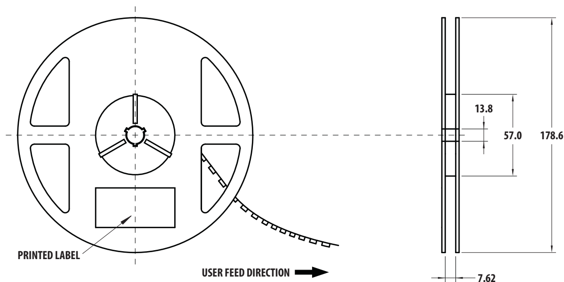
Figure 19: Reel Dimensions
