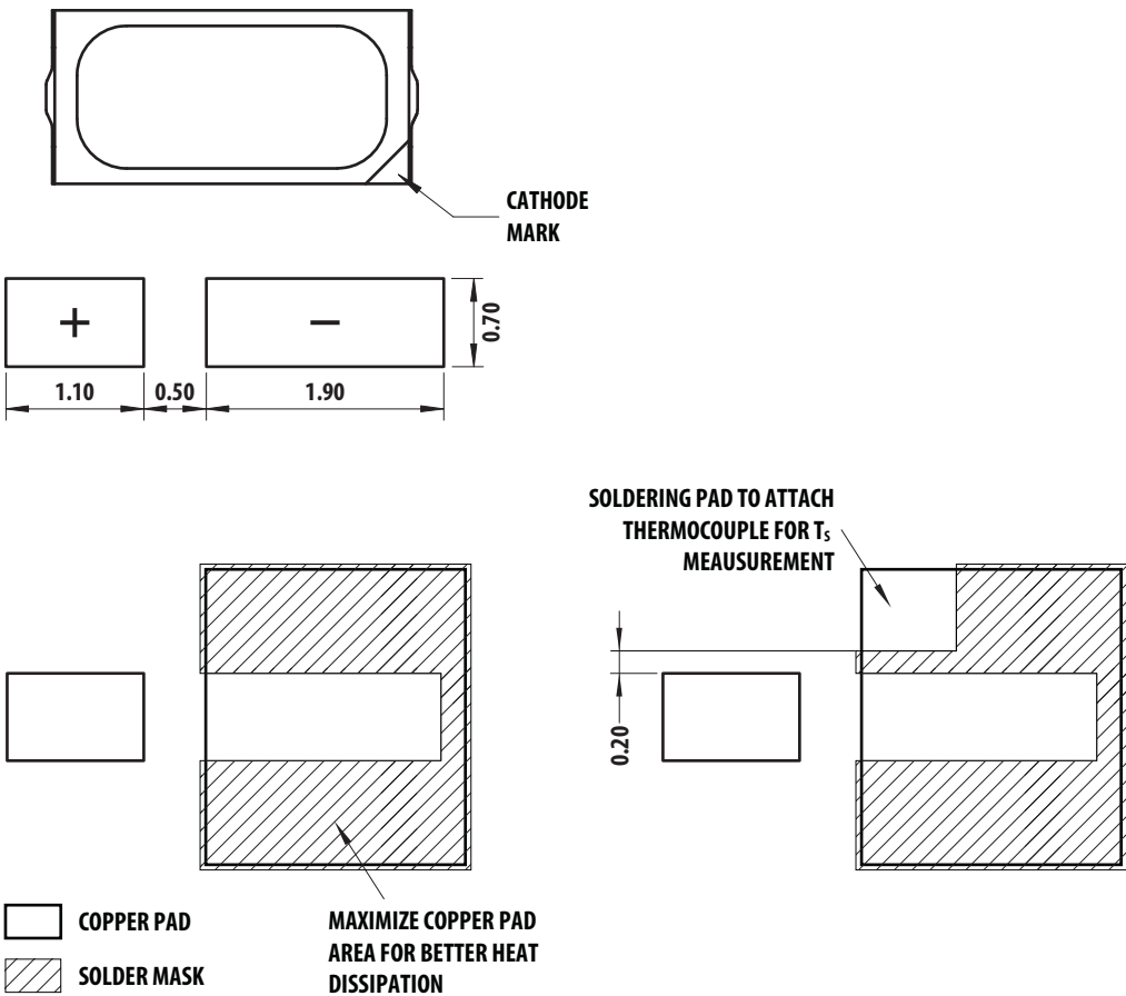
Figure 17: Recommended Soldering Pad Pattern
