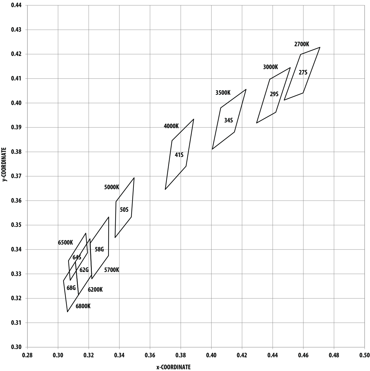
Figure 2: Chromaticity Diagram
