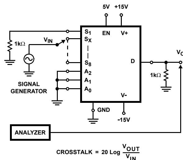
FIGURE 6. CROSSTALK
