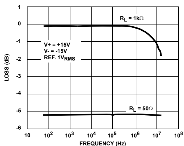
FIGURE 33. INSERTION LOSS vs FREQUENCY
