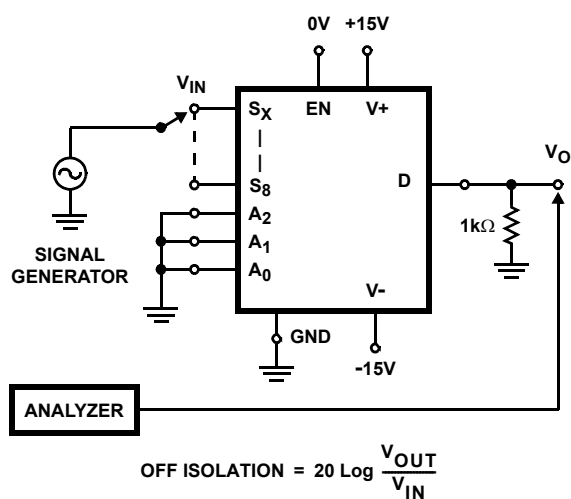
FIGURE 5. OFF ISOLATION
