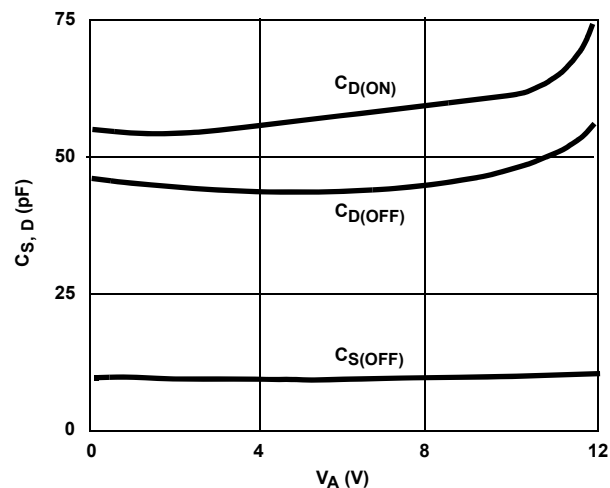
FIGURE 11. SOURCE/DRAIN CAPACITANCE vs ANALOG VOLTAGE (SINGLE 12V SUPPLY)
