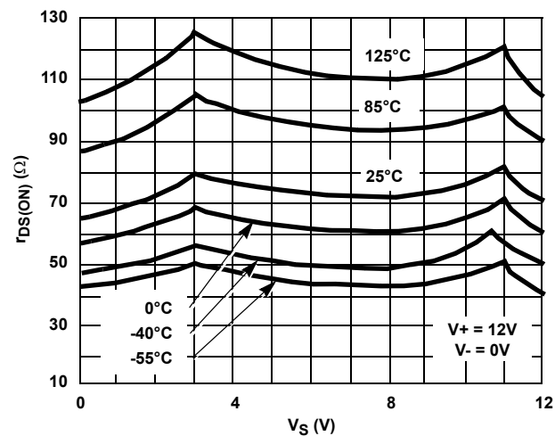
FIGURE 27. r_{DS(ON)} vs V_S AND TEMPERATURE (SINGLE SUPPLY)
