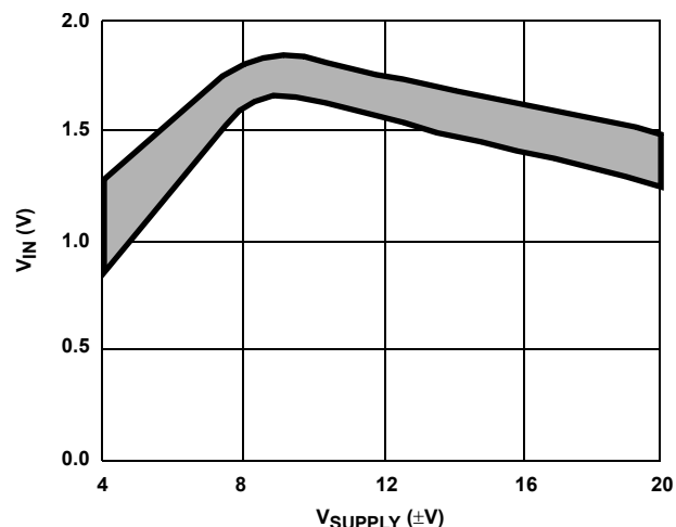
FIGURE 17. INPUT SWITCHING THRESHOLD vs SUPPLY VOLTAGE
