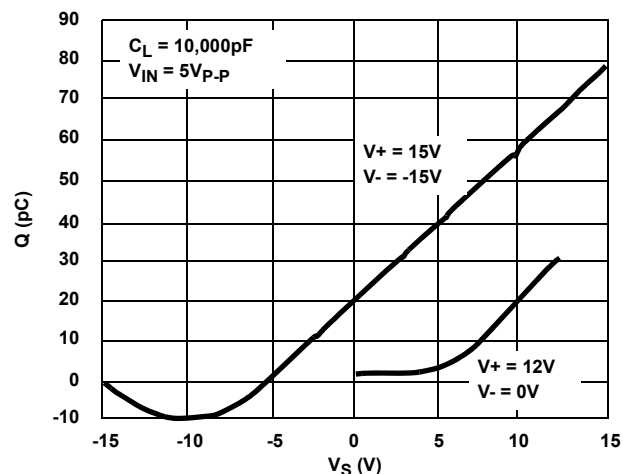
FIGURE 23. CHARGE INJECTION vs ANALOG VOLTAGE
