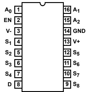
DG408 (PDIP, SOIC, TSSOP) TOP VIEW
