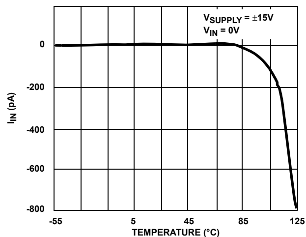
FIGURE 13. LOGIC INPUT CURRENT vs TEMPERATURE
