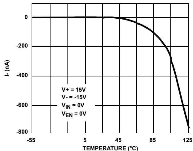
FIGURE 21. NEGATIVE SUPPLY CURRENT vs TEMPERATURE
