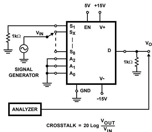
FIGURE 6. CROSSTALK
