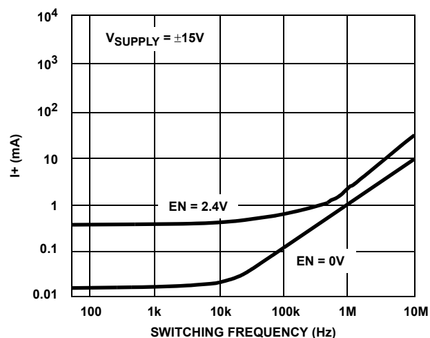
FIGURE 19. POSITIVE SUPPLY CURRENT vs SWITCHING FREQUENCY
