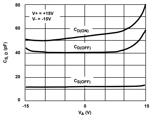
FIGURE 12. SOURCE/DRAIN CAPACITANCE vs ANALOG VOLTAGE
