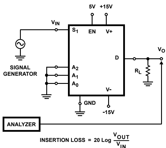
FIGURE 7. INSERTION LOSS
