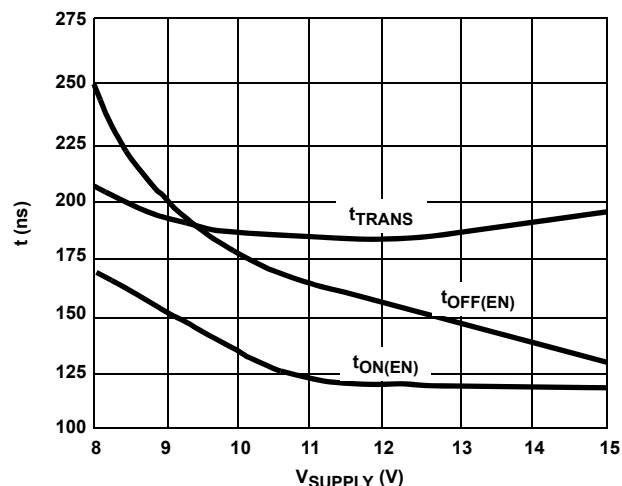
FIGURE 29. SWITCHING TIME vs SINGLE SUPPLY
