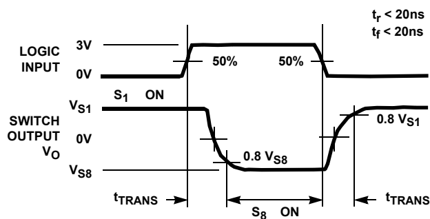
FIGURE 1C. MEASUREMENT POINTS
