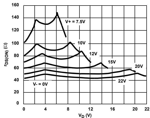
FIGURE 25. r_{DS(ON)} vs V_D (SINGLE SUPPLY)
