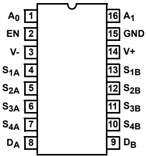
DG409 (PDIP, SOIC, TSSOP) TOP VIEW
