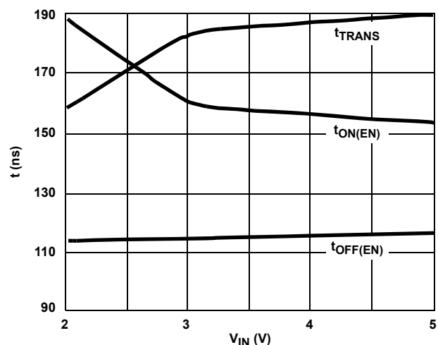
FIGURE 31. SWITCHING TIME vs V_{IN} (SINGLE SUPPLY)
