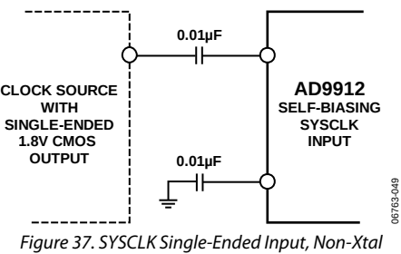
Figure 37. SYSCLK Single-Ended Input, Non-Xtal
