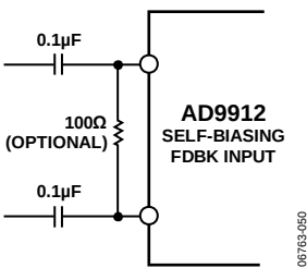
Figure 38. FDBK_IN Input
