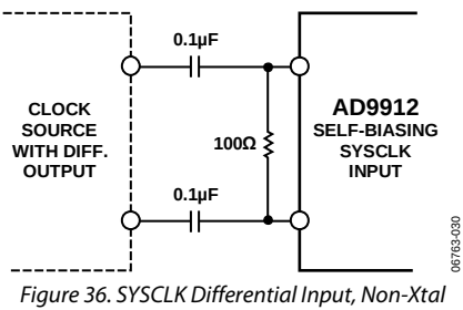
Figure 36. SYSCLK Differential Input, Non-Xtal
