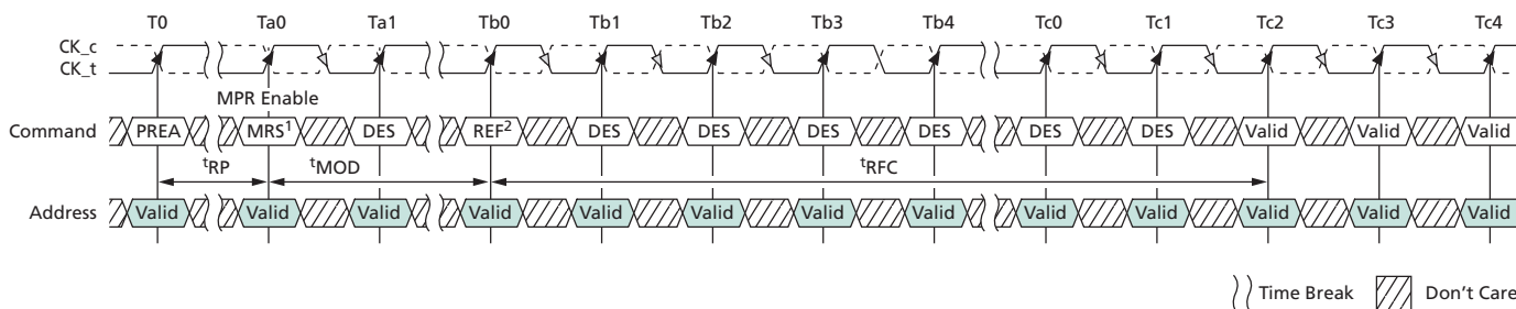
Figure 41: REFRESH Timing
