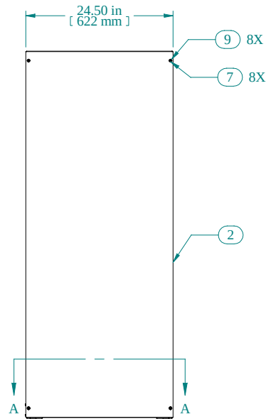
L.S. VIEW
