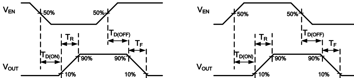
Figure 1. Voltage Waveforms: AP2501A (left), AP2511A (right)
