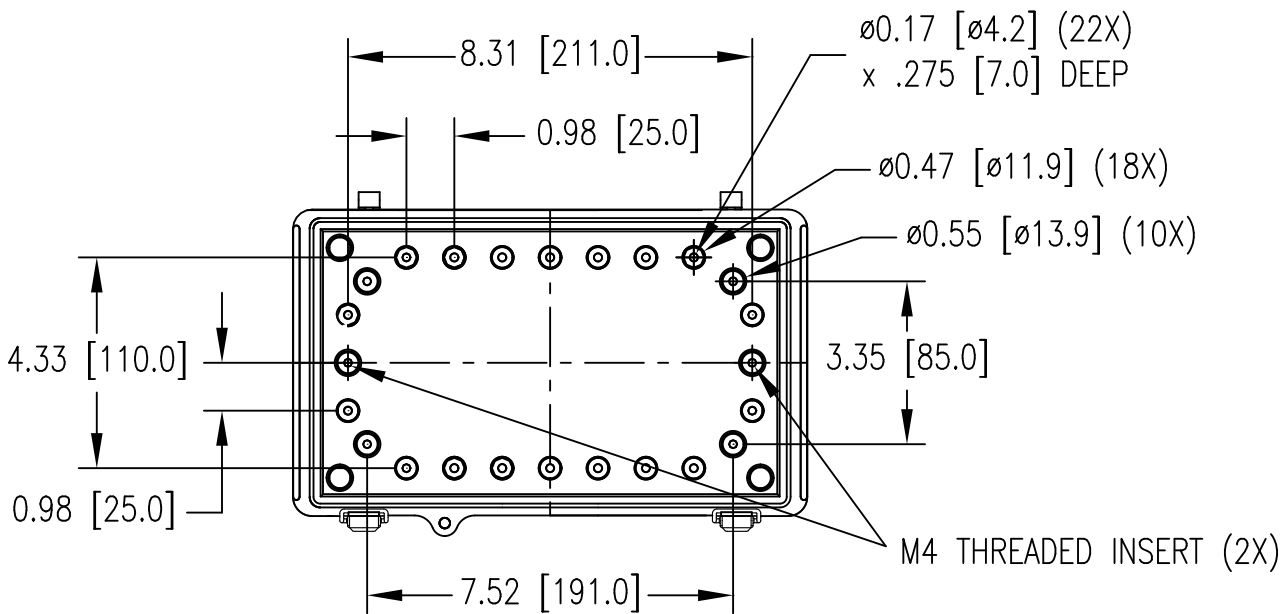
INSIDE VIEW OF BODY WITH COVER REMOVED
