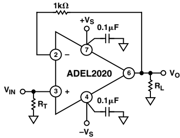
Figure 5. Connection Diagram for A_{VCL} = +1
