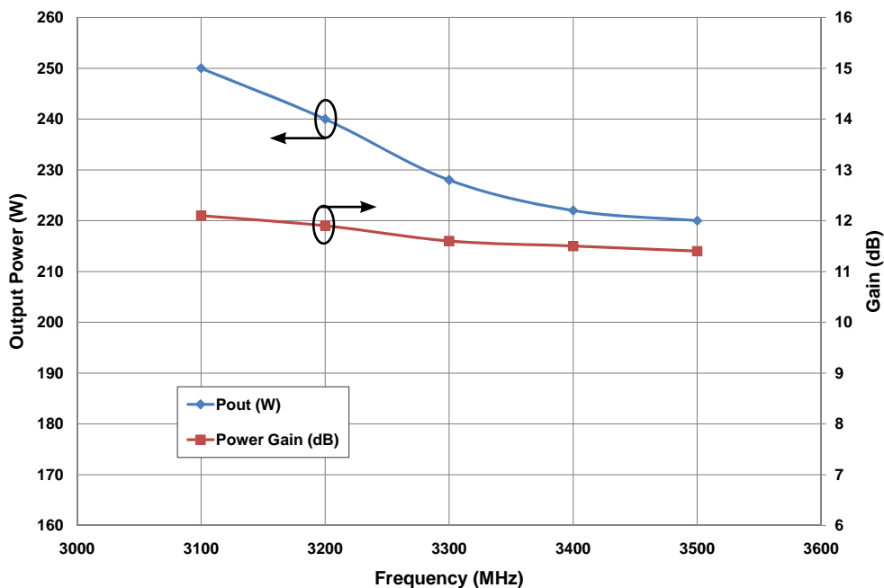
Typical Pulsed Output Power and Power Gain vs Frequency Measured in CGH35240-AMP Amplifier Circuit.
