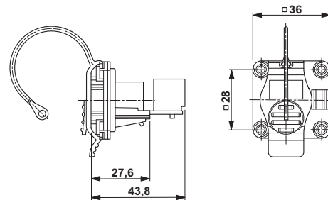
RJ45 panel mounting frame, IP67
