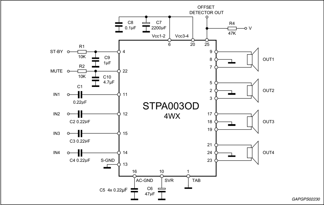
Figure 2. Standard test and application circuit (Flexiwatt25 with OD)
