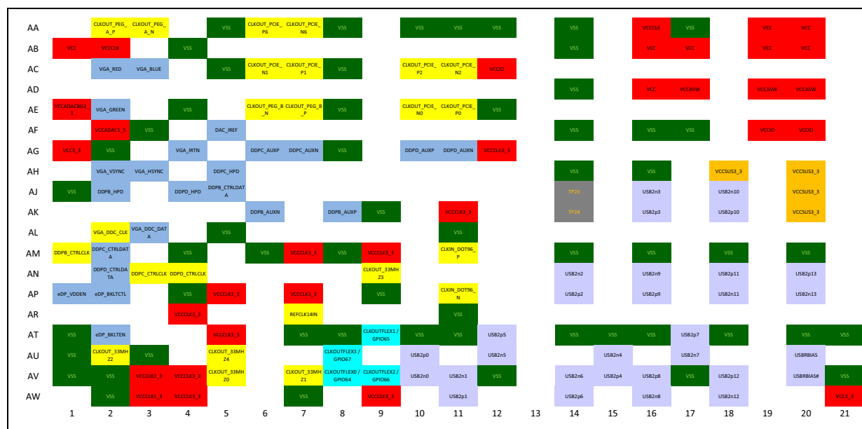
Figure 6-2. Desktop/Server PCH Ballout (Top View - Lower Left)
