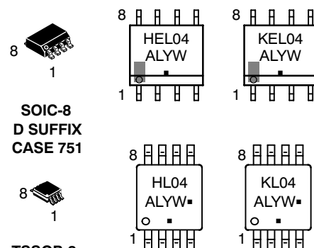
TSSOP-8 DT SUFFIX CASE 948R
