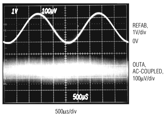
MAX537 REFERENCE FEEDTHROUGH AT 400Hz
