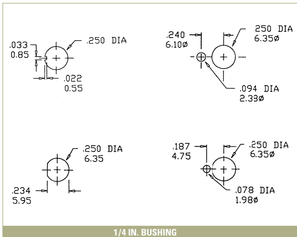
1/4 IN. BUSHING
