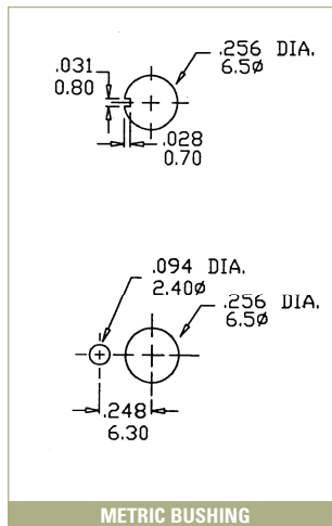
METRIC BUSHING
