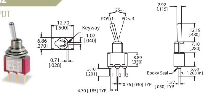
P.C. MOUNTING
