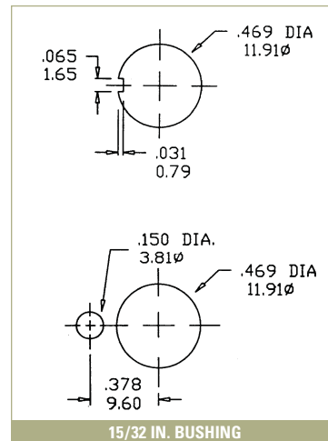
15/32 IN. BUSHING
