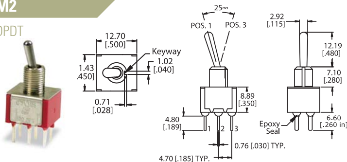
P.C. MOUNTING
