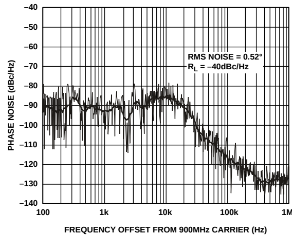
Figure 9. ADF4113 Integrated Phase Noise (900 MHz, 200 kHz, 20 kHz, Typical Lock Time: 400 \mu s)
