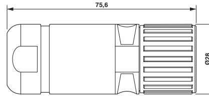
Dimensioned drawing
