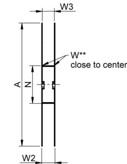
sectional drawing B-B
