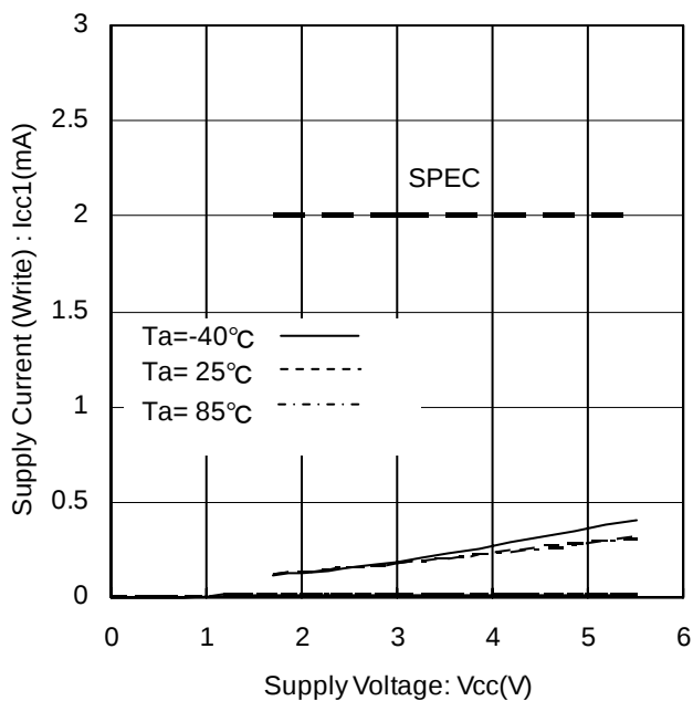
Figure 10. Supply Current (Write) vs Supply Voltage ( f_{SCL}=400kHz )
