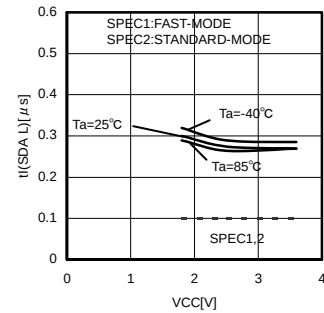
Fig.30 Noise Spike Width t_I(SDA L)
