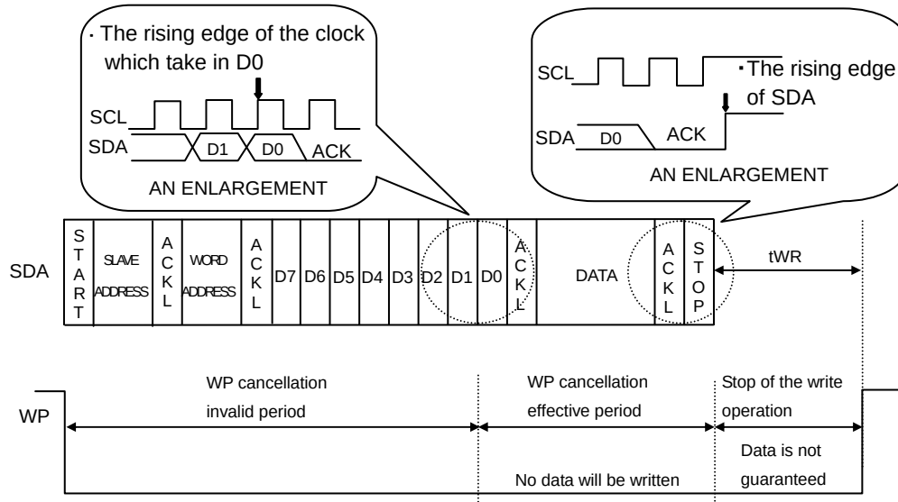
Fig.41 WP effective timing
