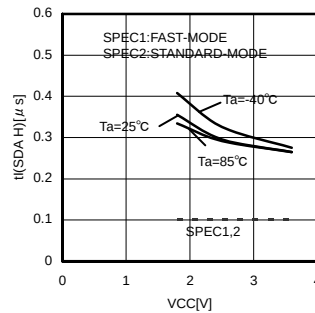
Fig.29 Noise Spike Width t_I(SDA H)
