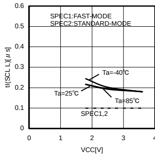
Fig.28 Noise Spike Width t_I(SCL L)
