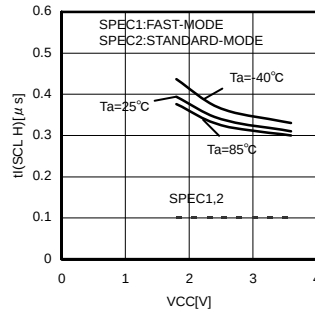
Fig.27 Noise Spike Width t_I(SCL H)
