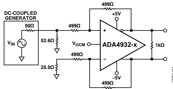
Figure 52. Equivalent Basic Test Circuit, G = 1
