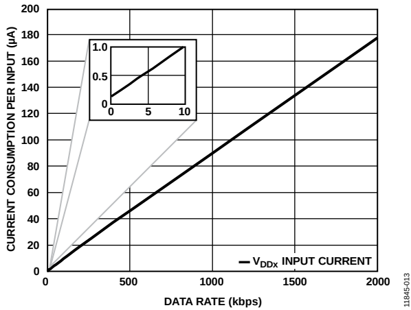
Figure 17. Current Consumption per Input vs. Data Rate for V_{DDX} = 3.3 V, EN_x = \text{High Operation}
