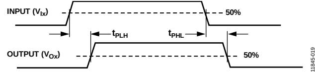
Figure 31. Propagation Delay Parameters
