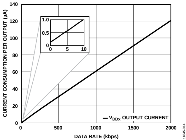
Figure 18. Current Consumption per Output vs. Data Rate for V_{DDX} = 3.3 V, EN_x = \text{High Operation}
